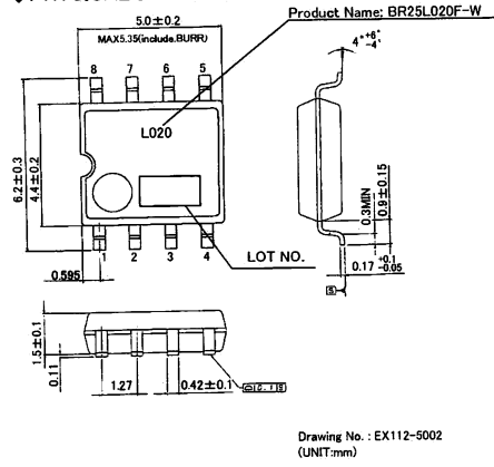
Fig4-(a) PHYSICAL DIMENSION SOP8 (BR25L020F-W)
