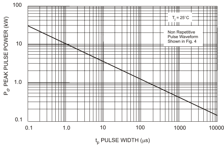
t_p PULSE WIDTH (µs) Fig. 3 Pulse Rating Curve
